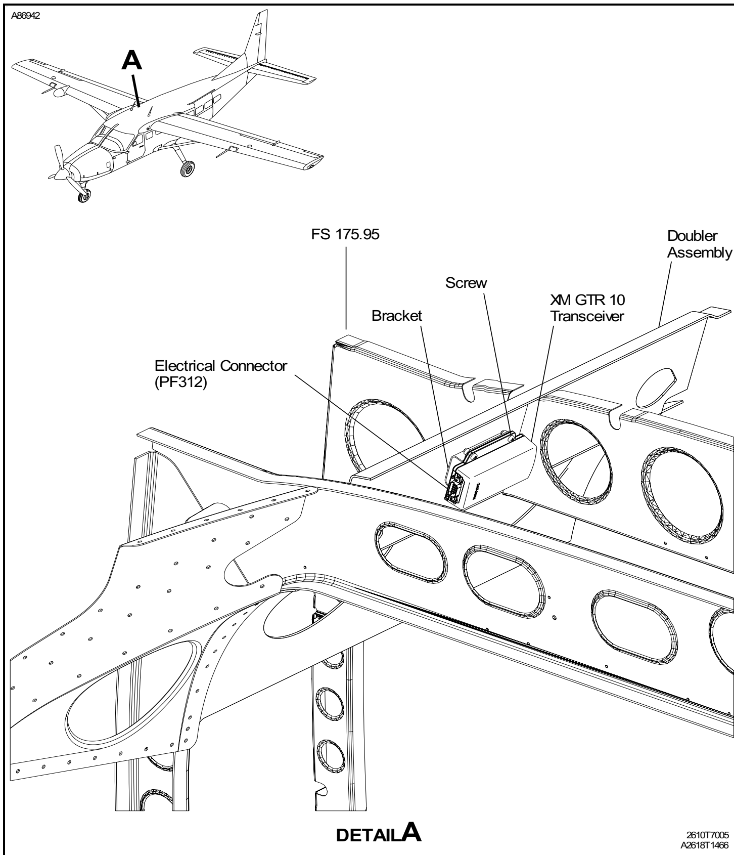
Figure 401 : Sheet 1 : XM GRT 10 Transceiver Installation
